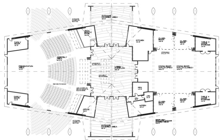
FLOOR PLAN 1" = 20'-0"
