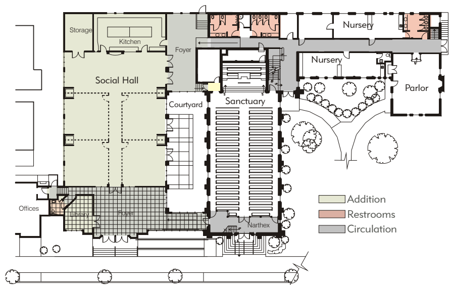
Main Floor Plan / Site Plan
